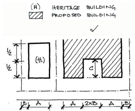
Figure SC6.3.4.6 Illustrates sympathetic building frontage rhythm. "B" is side setback; "C" (being the depth separation to get sympathetic building frontage rhythm) is 6m or \frac{1}{2} of "H" (heritage building depth)
